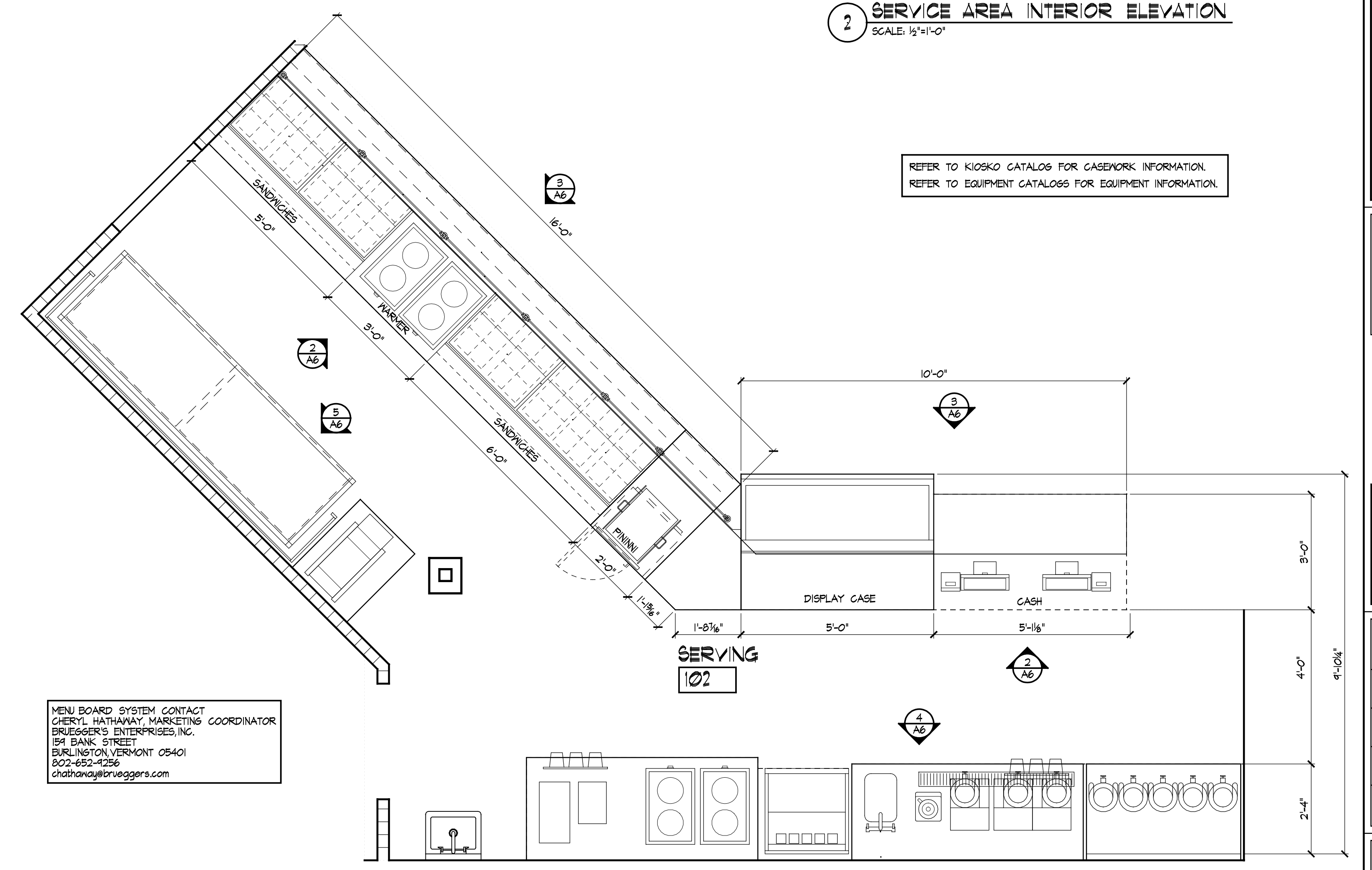
1 ENLARGED SERVICE AREA PLAN SCALE: 1/2" = 1'-0"
