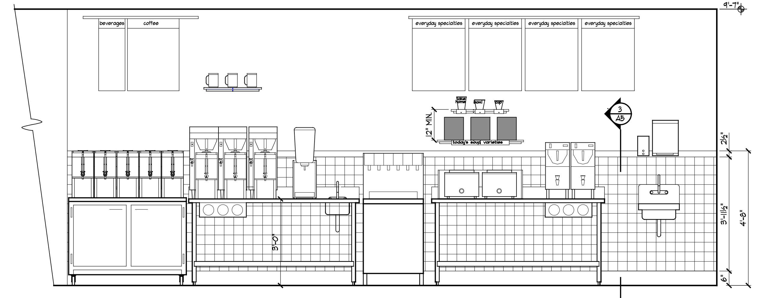
4 SERVICE AREA INTERIOR ELEVATION SCALE: 1/2" = 1'-0"
