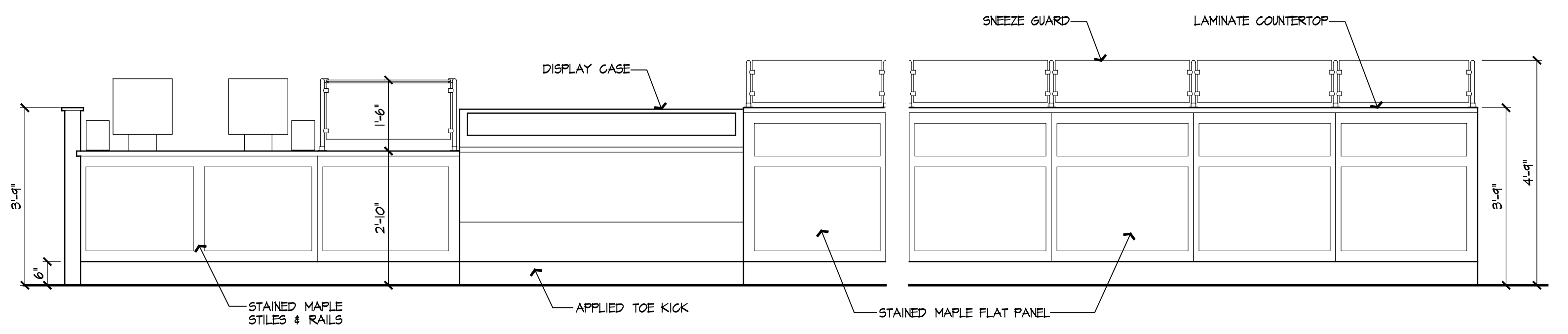
3 SERVICE AREA INTERIOR ELEVATION SCALE: 1/2" = 1'-0"
