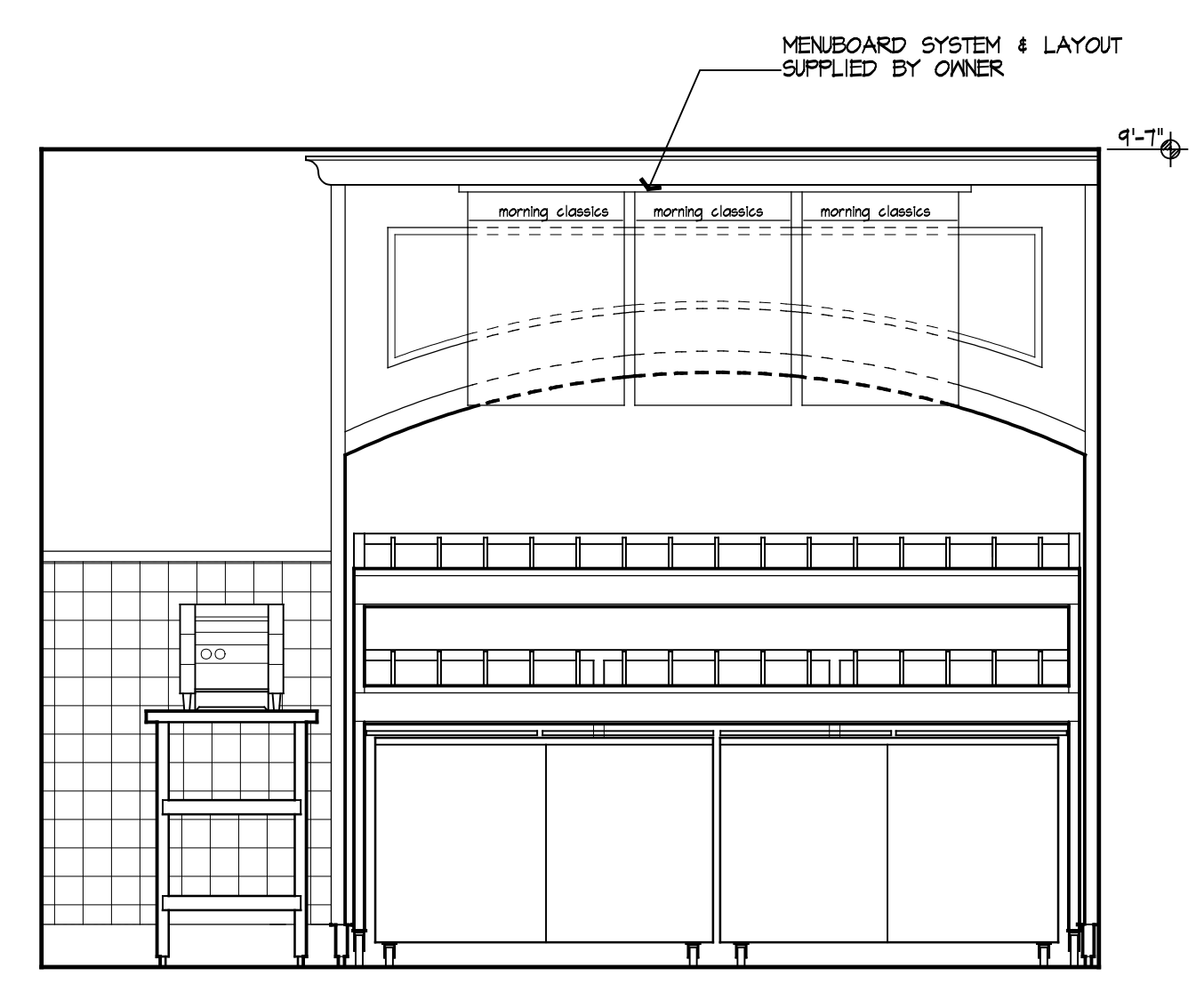
5 SERVICE AREA INTERIOR ELEVATION SCALE: 1/2" = 1'-0"
