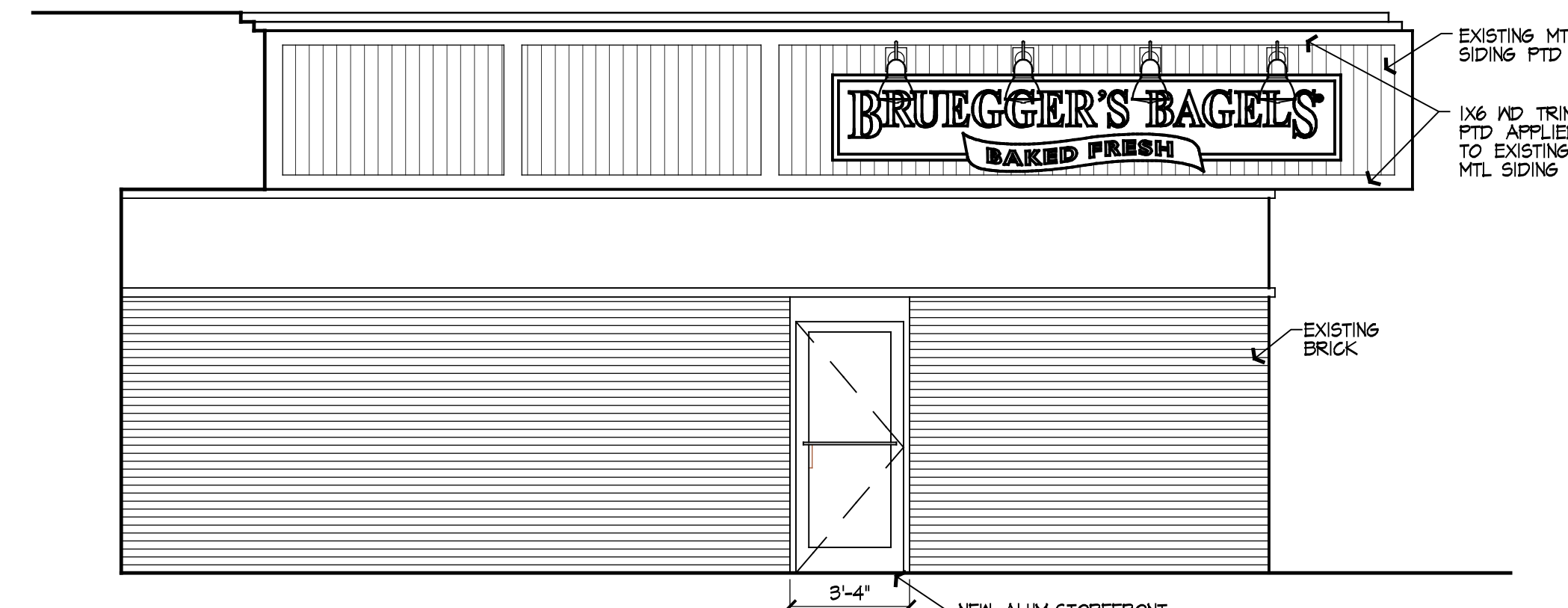
3 SOUTH ELEVATION SCALE: 1"=1'-0"
